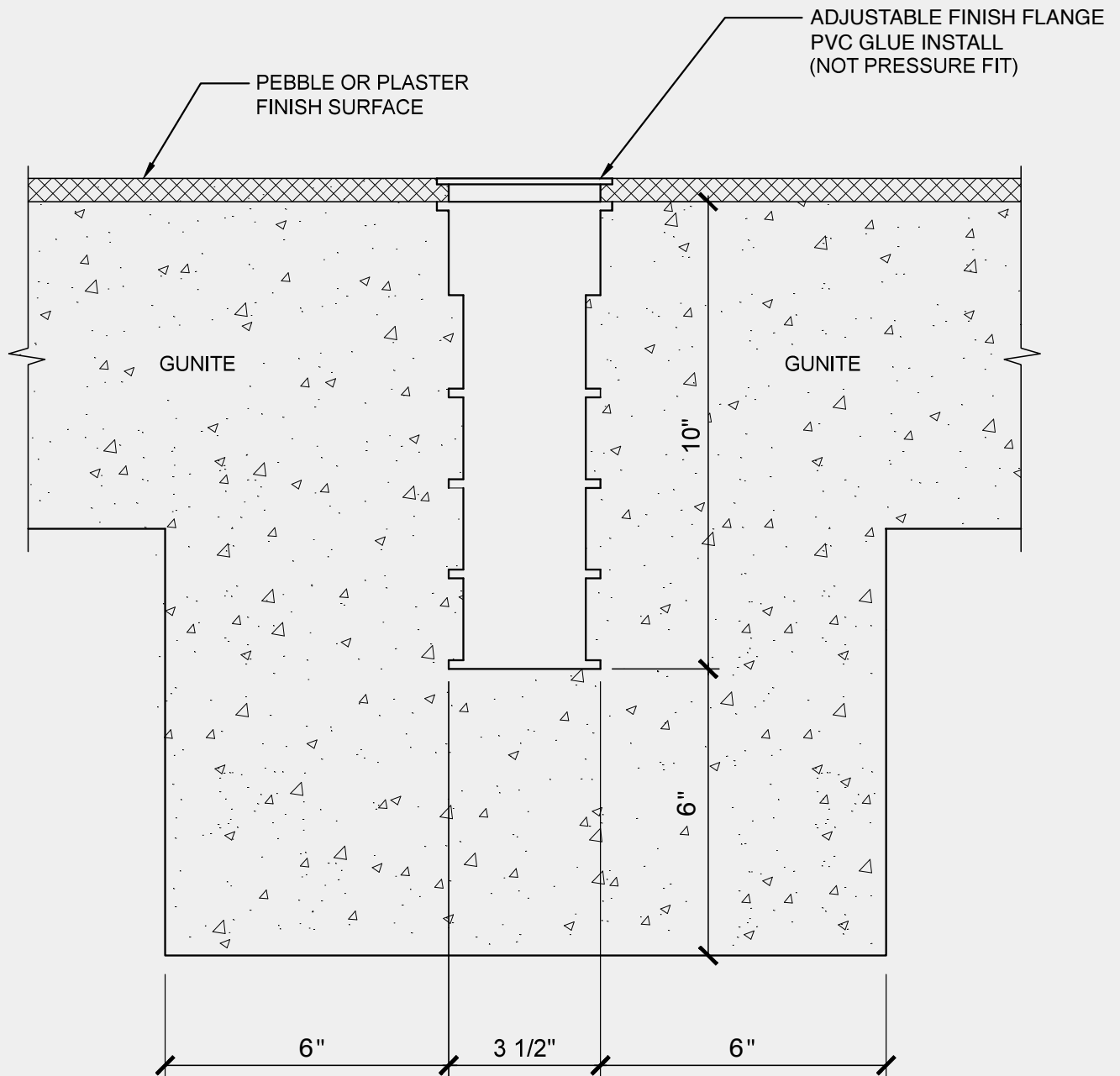
SANTA BARBARA DESIGNS INSTALLATION DIAGRAM 4-PC. POOL BAJA SHELF TUBE SYSTEM FOR 2" UMBRELLA POLES
